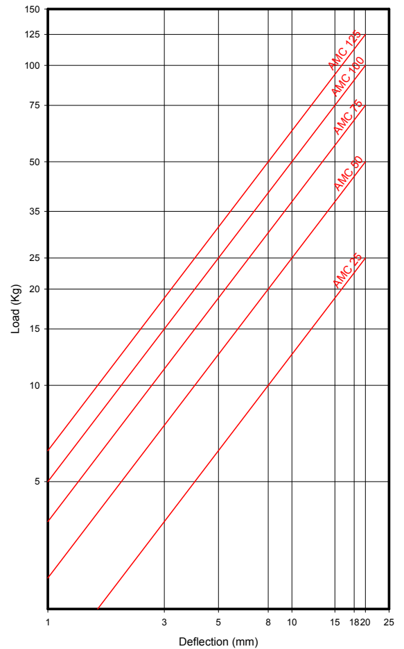
AMC LOAD DEFORMATION MECANOCAUCHO Medium Series type
