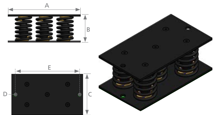
AMC LOAD DEFORMATION MECANOCAUCHO Type 5 AMC
