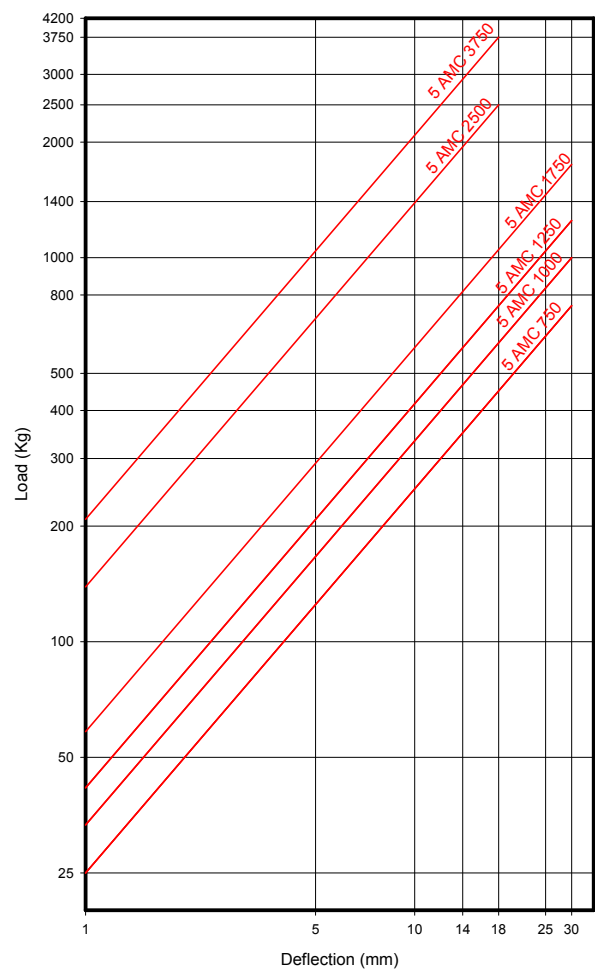
AMC LOAD DEFORMATION MECANOCAUCHO Type 5 AMC
