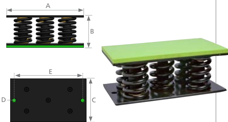
AMC Dynamic Natural Frequency range MECANOCAUCHO Type 5 AMC
