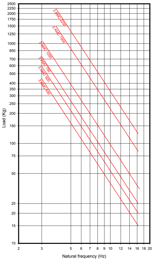
AMC Dynamic Natural Frequency range MECANOCAUCHO Type 3 AMC
