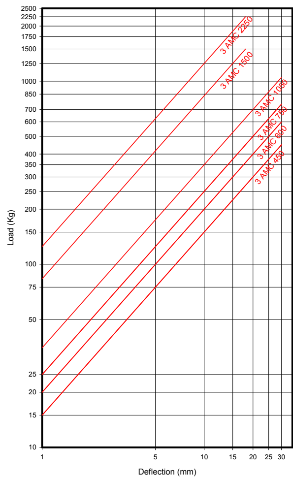
AMC LOAD DEFORMATION MECANOCAUCHO Type 3 AMC
