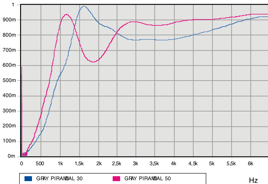
Absorption coefficient
