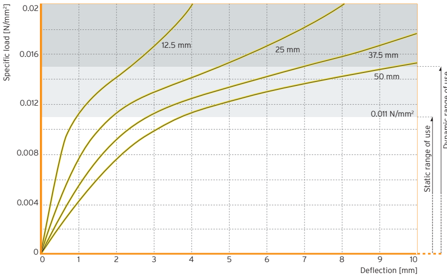
Figure 1: Quasistatic load deflection curve measured with a loading rate of 0.0011 N/mm²/s
