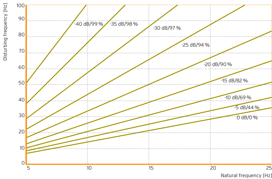
Figure 4: Reduction of the transmitted mechanical vibrations by implementation of an elastic bearing consisting of Sylomer® SR 11
