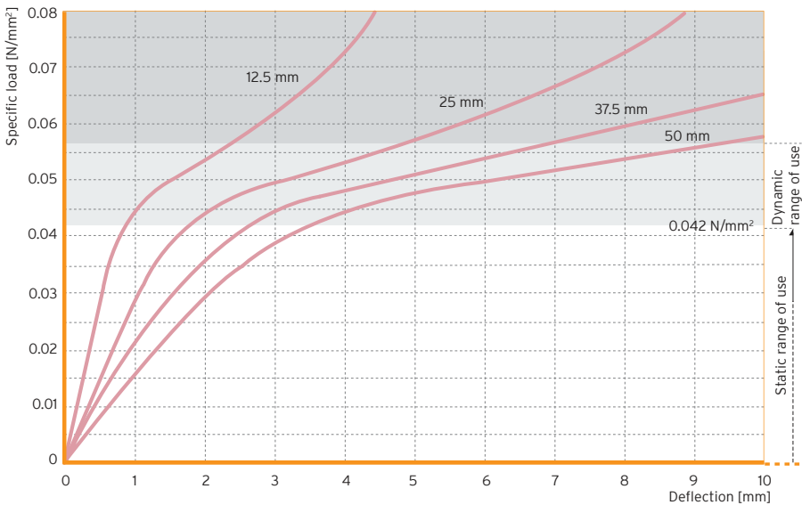
Figure 1: Quasistatic load deflection curve measured with a loading rate of 0.0042 N/mm²/s
