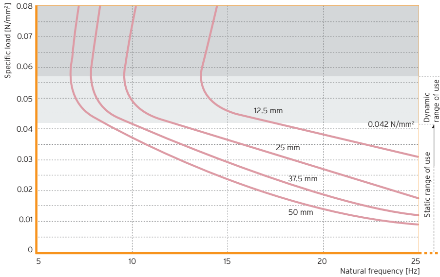
Figure 3: Natural frequency of a single-degree-of-freedom system (SDOF system) consisting of a fixed mass and an elastic bearing consisting of Sylomer® SR 42 based on a stiff subgrade
