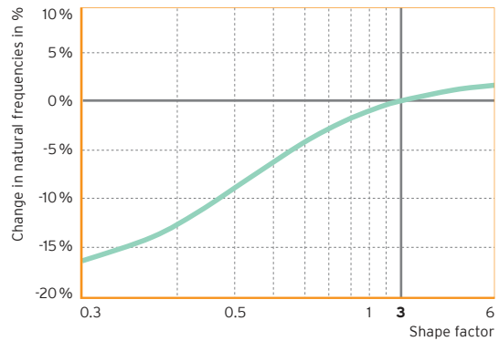
Fig. 8: Natural frequency 5 in relation to the shape factor
