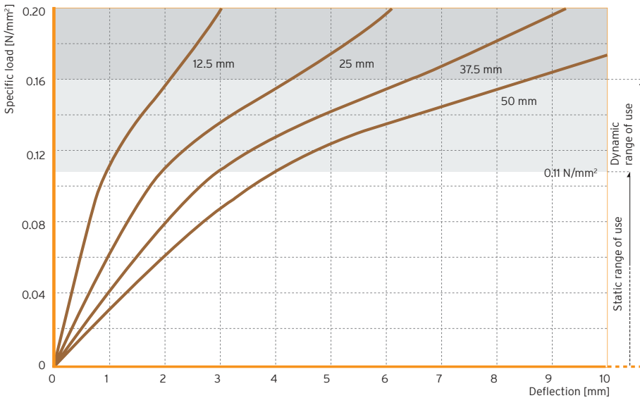
Figure 1: Quasistatic load deflection curve measured with a loading rate of 0.011 N/mm²/s
