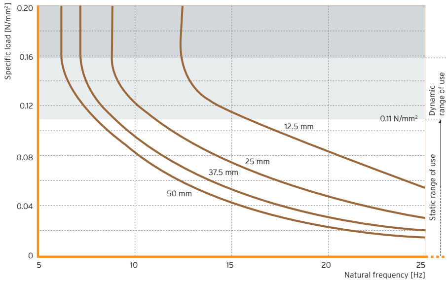
Figure 3: Natural frequency of a single-degree-of-freedom system (SDOF system) consisting of a fixed mass and an elastic bearing consisting of Sylomer® SR 110 based on a stiff subgrade
