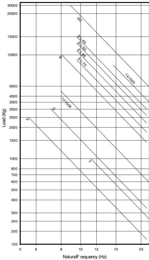
NATURAL FREQUENCY HIGH LOAD MOUNTS
