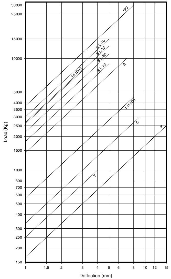
LOAD DEFLECTION CURVES HIGH LOAD MOUNTS
