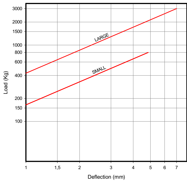
LOAD-DEFLECTION CURVE TRANSFORMER MOUNTS
