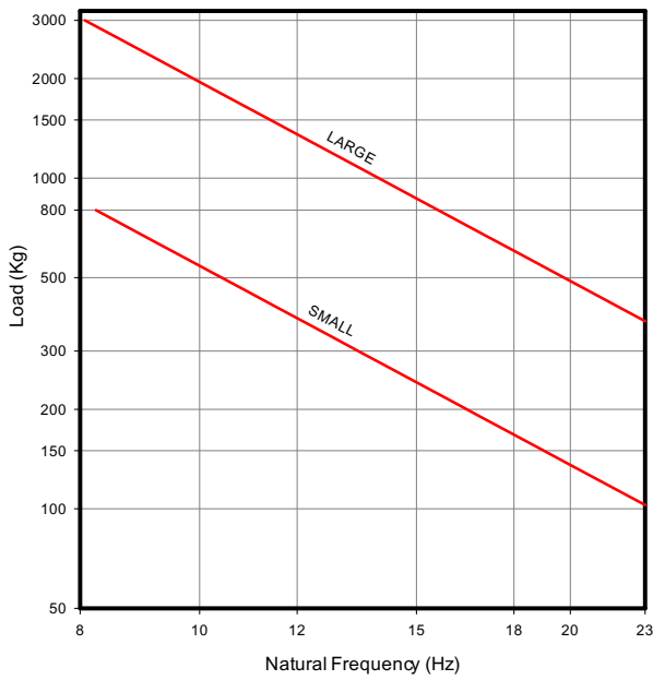
NATURAL FREQUENCY TRANSFORMER MOUNTS
