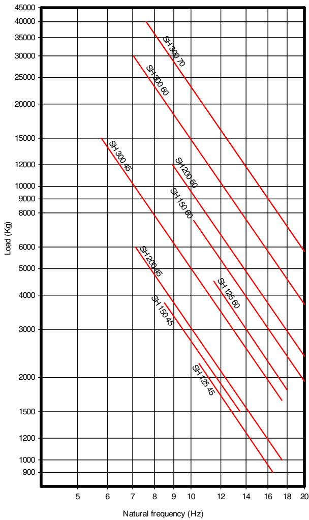
NATURAL FREQUENCIES AMC MECANOCAUCHO SH
