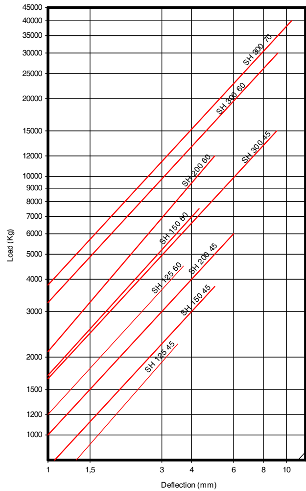
LOAD DEFLECTION GRAPHS AMC MECANOCAUCHO SH
