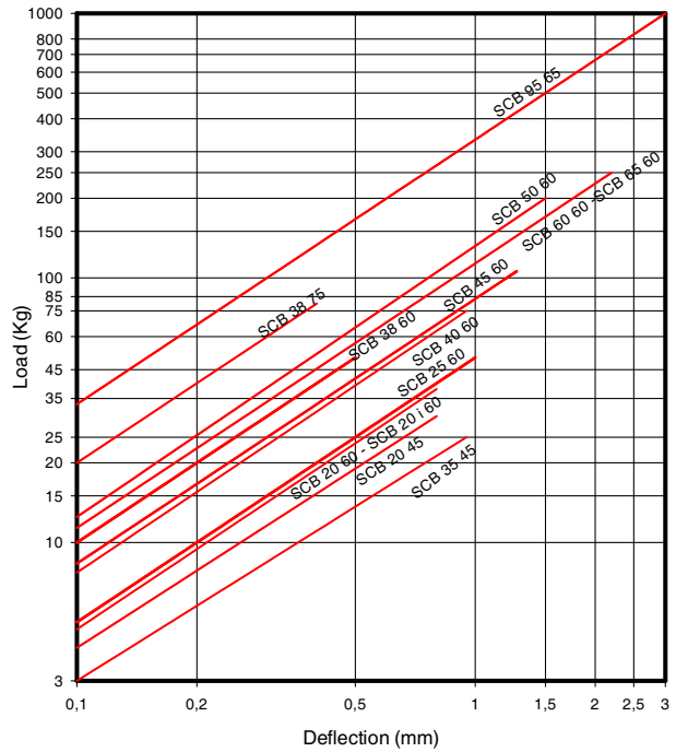
AMC LOAD DEFLECTION CURVES MECANOCAUCHO® SCB
