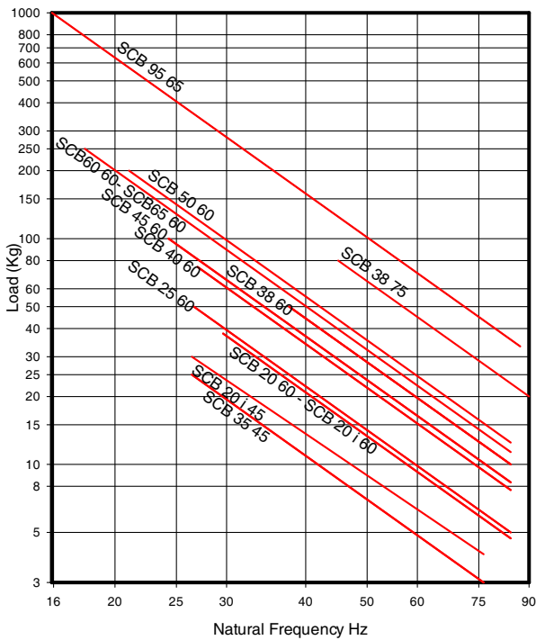
AMC NATURAL FREQUENCY MECANOCAUCHO® SCB
